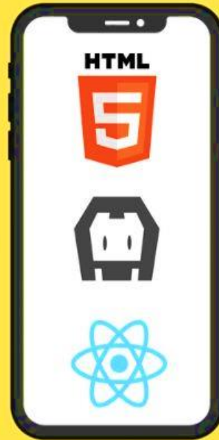
Hybrid Apps
